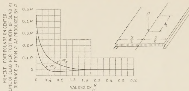
FIGURE 8.—BENDING MOMENTS ON CENTER LINE OF SIMPLY SUPPORTED SLAB AT DISTANCE y FROM P AS PRODUCED BY P , FOR SLABS HAVING MAIN REINFORCEMENT PARALLEL TO THE DIRECTION OF TRAFFIC.
